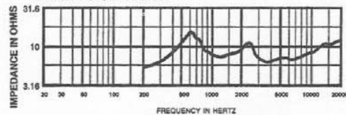
FIGURE 6 — Impedance Response, Plane-Wave Tube, DH2As1 8-Ohm Driver
