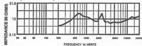
FIGURE 8 — Impedance Response, 2-Inch Plane-Wave Tube
