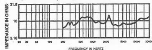
FIGURE 7 — Impedance Response, on HP640 Horn
