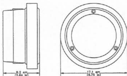
FIGURE 3 — Dimensions
